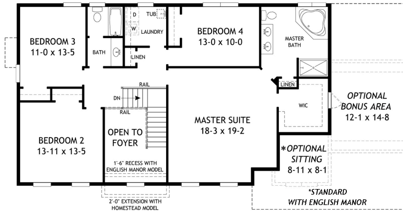
SECOND FLOOR
